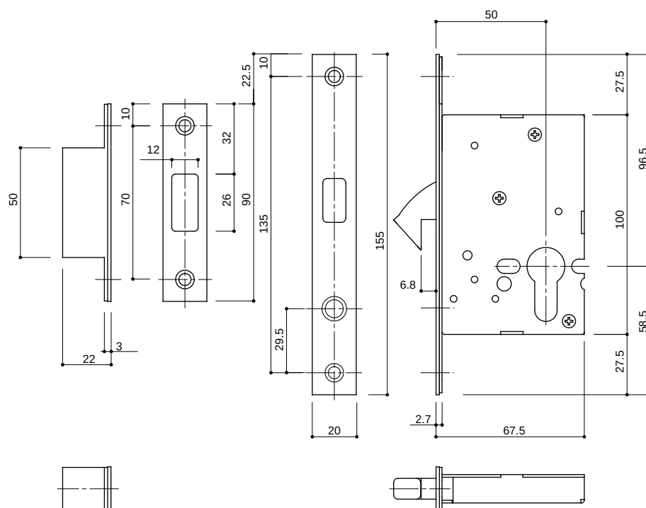
Cross Section Diagrams & Measurements for KZK2 Lock Case KZK2 鎖匣尺寸圖/開孔圖
