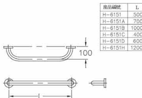
H-6151C 400長×100寬mm $2,800 H-6151 500長×100寬mm $2,900 H-6151D 600長×100寬mm $3,100 H-6151A 700長×100寬mm $3,200 H-6151B 1000長×100寬mm $3,800 H-6151H 1200長×100寬mm $4,100 C型扶手 1 1/4" \phi 註：附膨脹螺絲6支 材質：不銹鋼#304 (管徑 \phi 31.8mm)
