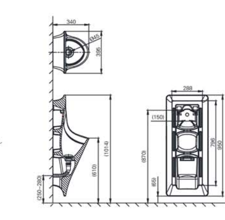
Back Inlet Urinal Size:395x340x950mm Included:Sensor 後進水小便斗 尺寸: 395x340x950mm 自帶感應器
