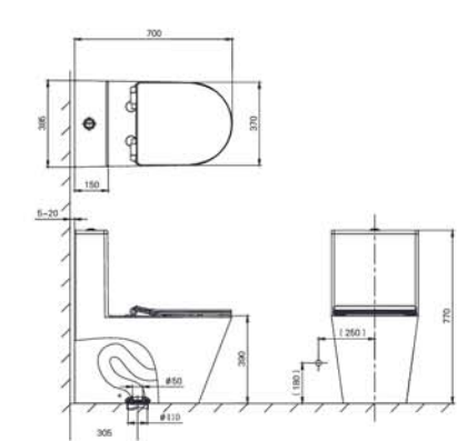
One-Piece Toilet Size:700x385x770mm Cover Seat: Slim UF Soft-closing Rough-in: 305mm Dual Flush: 3.5/5L Flush System:Siphon 連體座便器 尺寸: 700x385x770mm 蓋板: UF緩降薄蓋板 坑距: 305mm 名義用水量: 3.5/5L 沖水系統:虹吸
