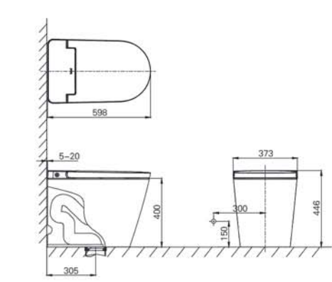
One-Piece Toilet Size: 598x373x446mm Cover Seat: Slim UF Soft-closing Rough-in : 305mm Dual Flush: 4.2/6L Flush System:Siphon 一體座便器 尺寸: 598x373x446mm 蓋板: UF緩降薄蓋板 坑距: 305mm 名義用水量: 4.2/6L 沖水系統:虹吸
