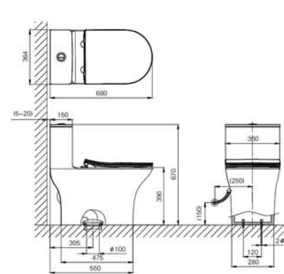
One-Piece Toilet Size:680x360x670mm Cover Seat: PP Soft-closing Rough-in: 305mm Dual Flush: 3/4.5L Flush System:Vortical Siphon 連體座便器 尺寸: 680x360x670mm 蓋板: PP緩降蓋板 坑距: 305mm 名義用水量: 3/4.5L 沖水系統:旋渦虹吸
