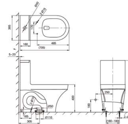
One-Piece Toilet Size:705x365x750mm Cover Seat: Slim UF Soft-closing Rough-in: 305mm Dual Flush: 3.5/5L Flush System:Siphon 連體座便器 尺寸: 705x365x750mm 蓋板: UF緩降薄蓋板 坑距: 305mm 名義用水量: 3.5/5L 沖水系統:虹吸
