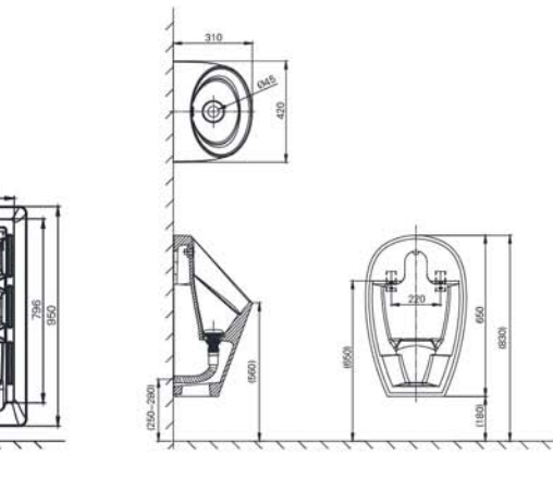
Back Inlet Urinal Size:420x310x650mm Included: Sensor 後進水小便斗 尺寸: 420x310x650mm 自帶感應器
