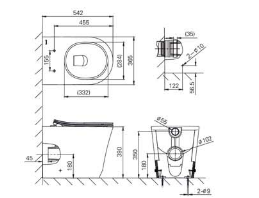
Floorstanding Toilet Size: 542x365x390mm Cover Seat: Slim UF Soft-closing Rough-in : H=180mm(P-Trap Height) Recommended Products: In-Wall Tank System:(NCD03C) Flush System:Wash Down 落地式座便器 尺寸: 542x365x390mm 蓋板: UF緩降薄蓋板 坑距: H=180mm (P排) 可搭配NCD03C隱藏式水箱使用 沖水系統:直沖
